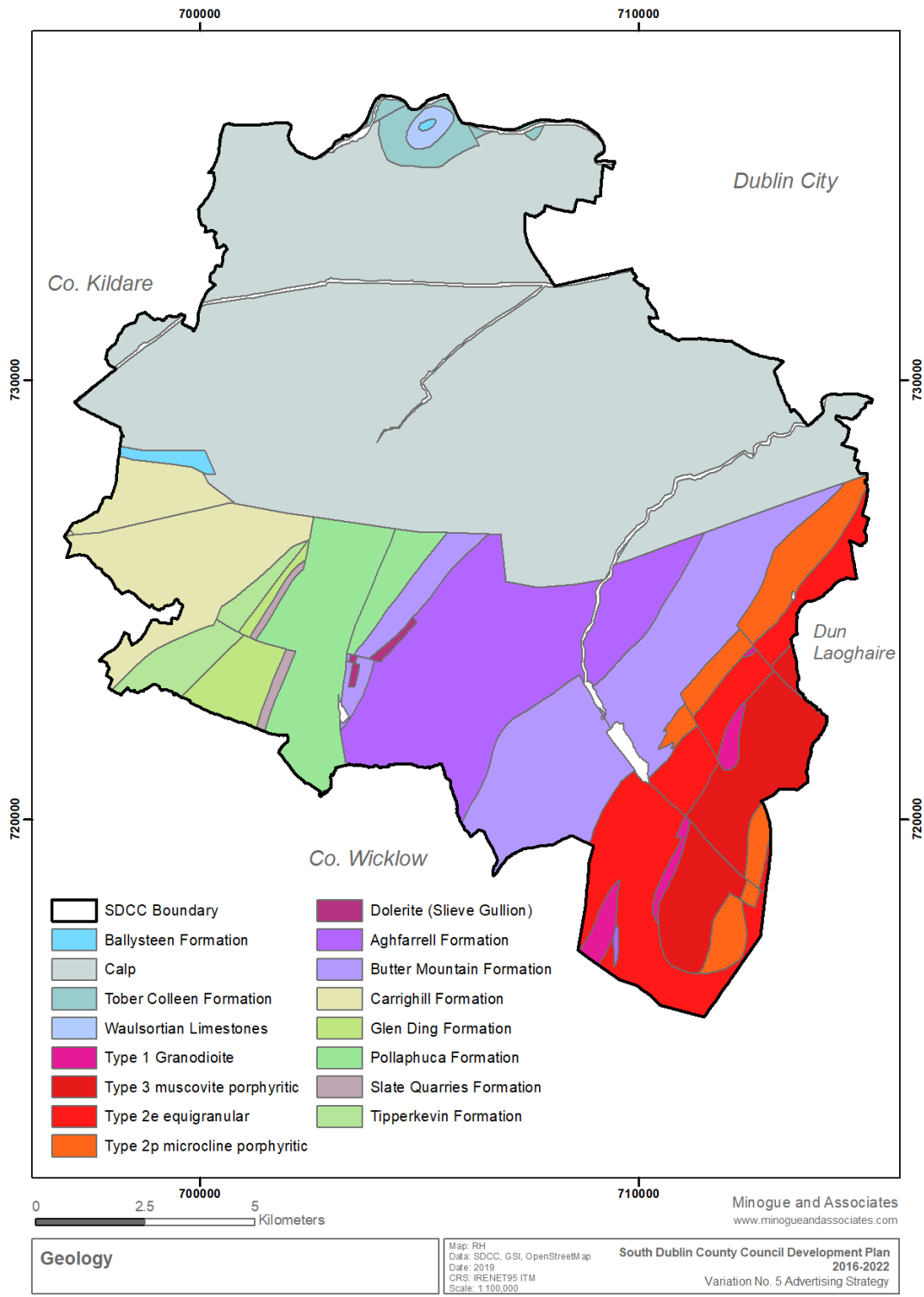
FIGURE 7 BEDROCK GEOLOGY
